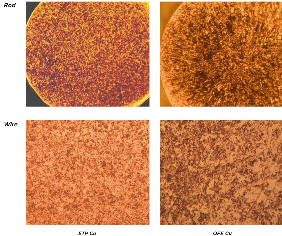
Figure 1. Microstructure of ETP Copper and OFE Copper
